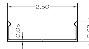
15- BCE-2564 FACE COVER - ALUMINUM ALLOY 6063-T5
