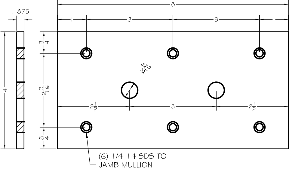
#37 - 3/16" 4 X 8 ASTM A36 JAMB REINF. STEEL PLATE
