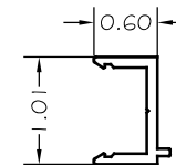
12- PHX-611 EXTERIOR FILLER BASE ALUMINUM ALLOY 6063-T6
