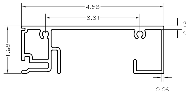
7- PHX-606 EXPANSION BOTTOM RAIL ALUMINUM ALLOY 6063-T6
