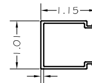
11- PHX-610 IG EXTERIOR FILLER COVER ALUMINUM ALLOY 6063-T6
